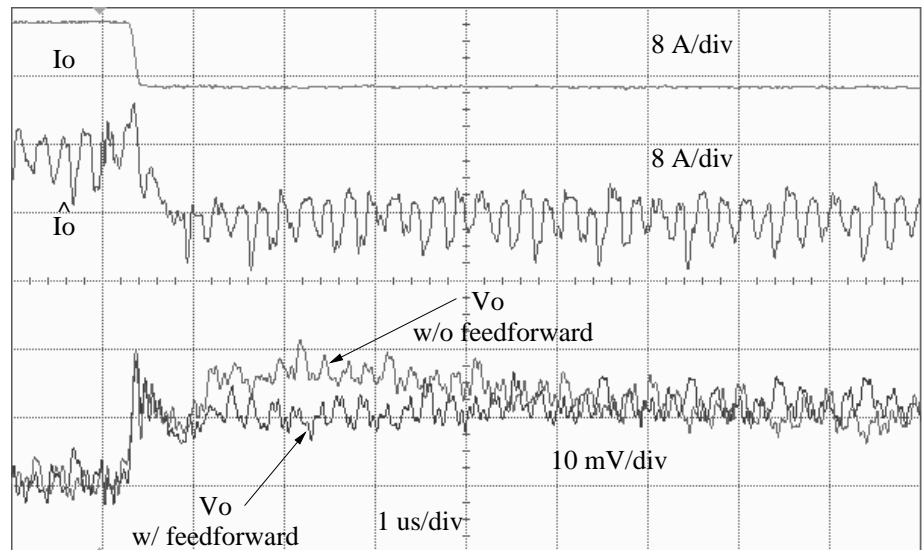
Figure 2.13: Experimental 8 A unloading transient, from 68 A to 60 A, with corresponding estimated load current, with and without load-current feedforward.
