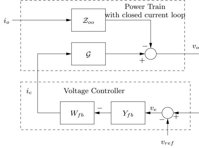
Figure 2.5: Block diagram of current-mode load-line control with finite DC gain compensator Y_{fb} .
