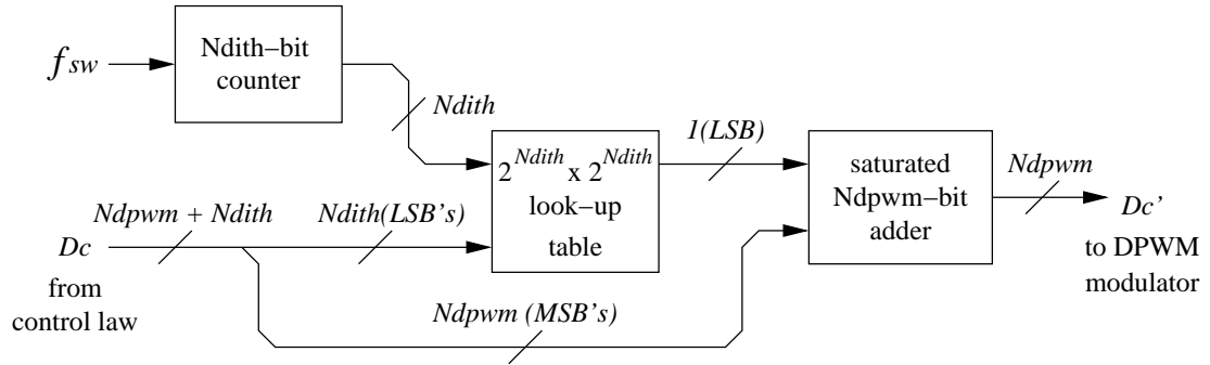
Figure 3.7: Structure for adding arbitrary dither patterns to the duty ratio, boosting the effective DPWM resolution by N_{dith} bits.
