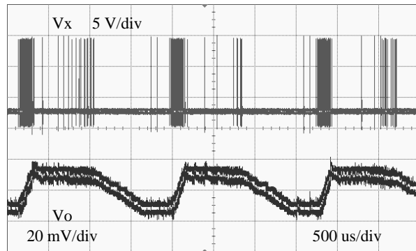
(d) Pulse skipping ( I_o = 0.1 A). Periodic behavior at about 560 Hz.
