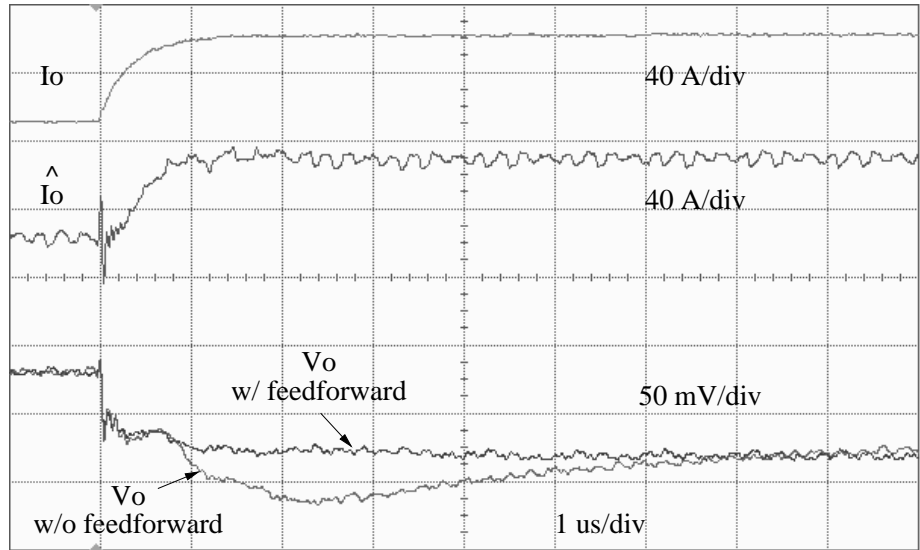
(a) Loading step from 60 A to 112 A
