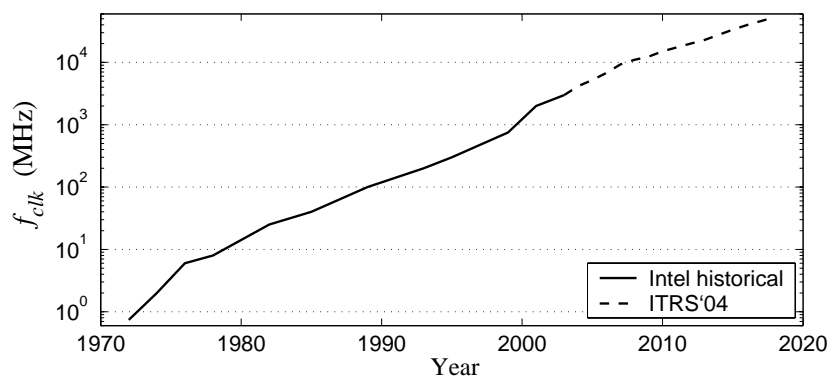
(b) Microprocessor clock frequency. (Sources: [105, 29, 30])
