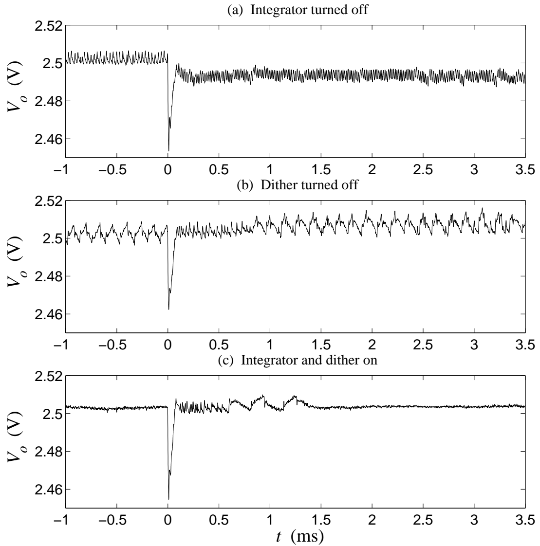
Figure 3.12: Experimental steady-state behavior and transient response of the prototype buck converter with and without integral feedback and dither. Load current steps from 0.5 A to 12 A at t = 0 .
