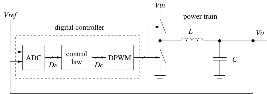
Figure 3.1: Basic block diagram of a digitally-controlled PWM buck converter.
