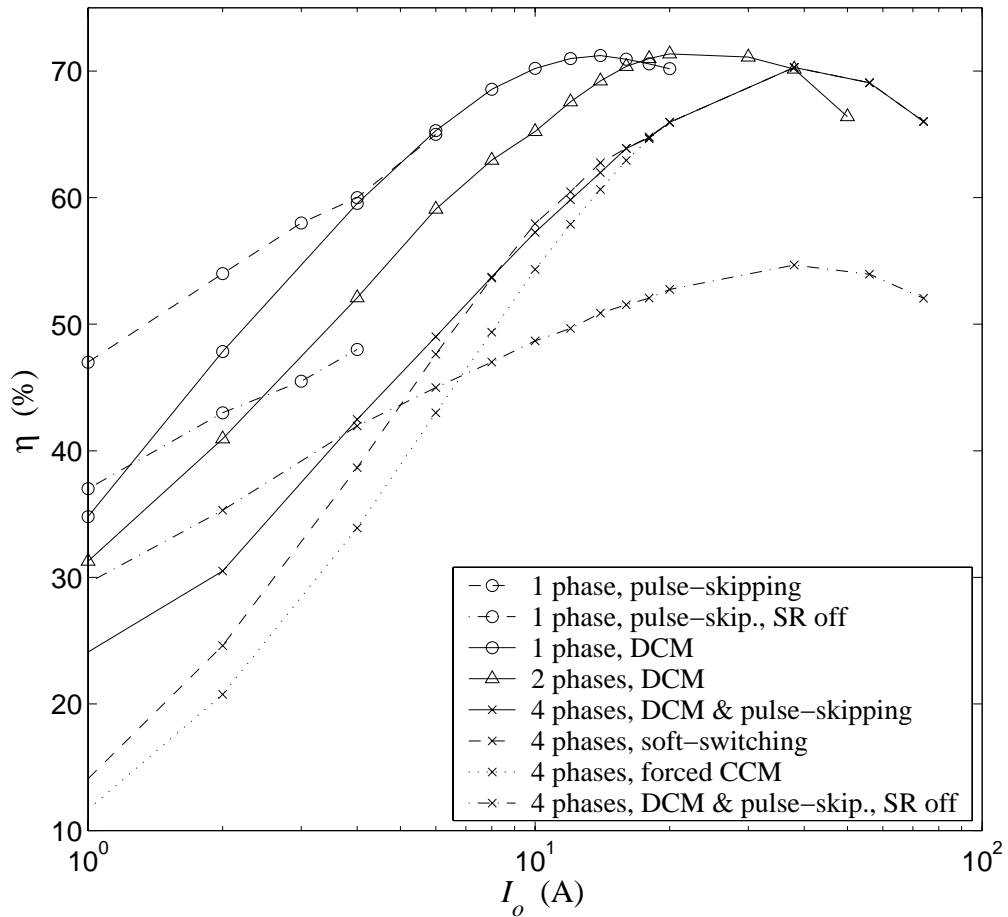
Figure 4.12: Converter efficiency \eta versus load current I_o for different number of phases and modes of operation.
