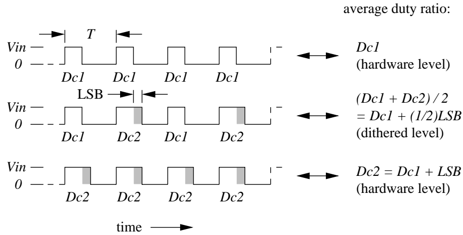
Figure 3.5: Use of switching waveform dither to realize a (1/2)LSB effective DPWM level (1-bit dither).
