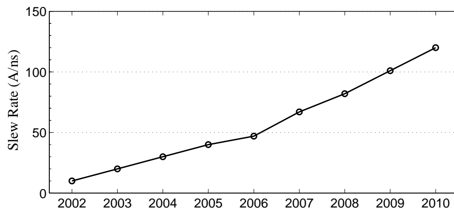
(d) Microprocessor current slew rate. (Source: [113])
