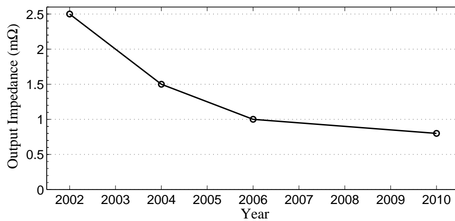
(e) Microprocessor power supply output impedance. (Source: [43])
