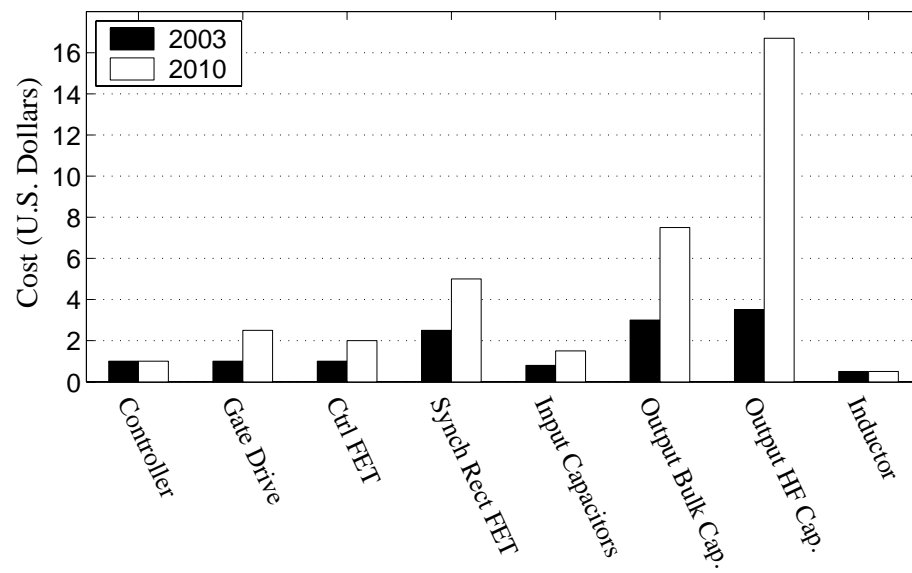
Figure 1.2: Microprocessor voltage regulator cost breakdown, assuming use of present-day multi-phase buck topology in future. (Source: [113])
