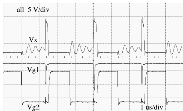
(c) DCM operation with gated synchronous rectifier ( I_o = 5 A).
