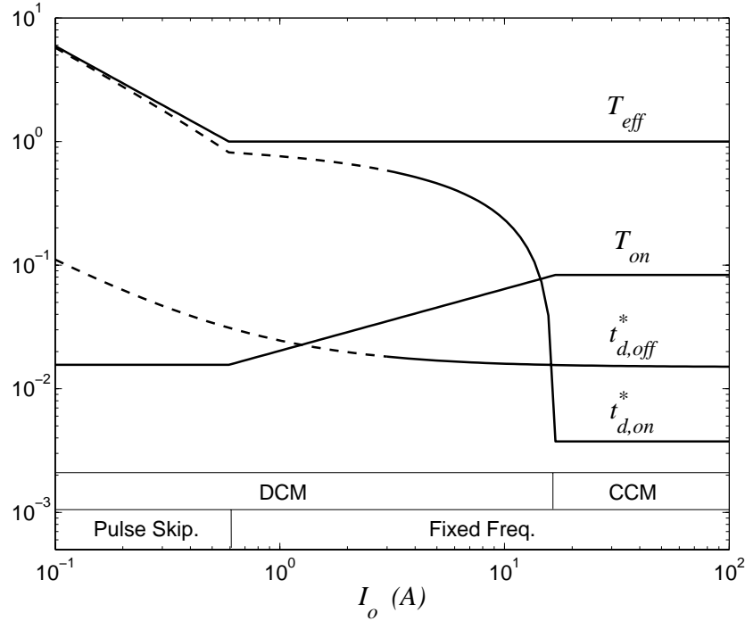
Figure 4.2: Timing parameters of the buck-converter control switch and synchronous rectifier for different modes of operation. All parameters are normalized by the fixed-frequency switching period T , and both axes are logarithmic.
