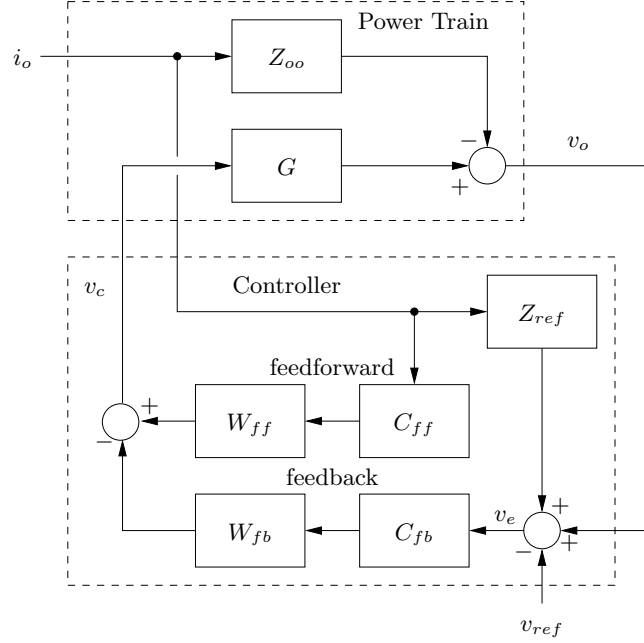
Figure 2.6: Voltage-mode load-line control block diagram with load-current feedforward.
