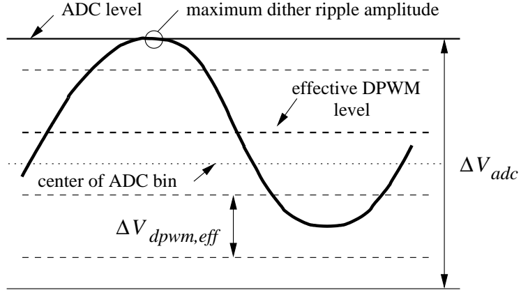
Figure 3.8: Maximum dither ripple amplitude constraint. Illustrated case is for N_{dpwm,eff} = N_{adc} + 2 .
