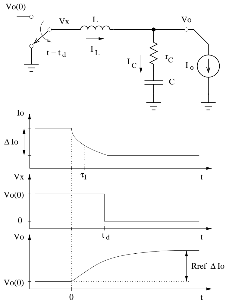
Figure 2.7: Buck converter transient response model for a large unloading current step.
