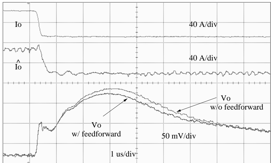
(b) Unloading step from 112 A to 60 A
