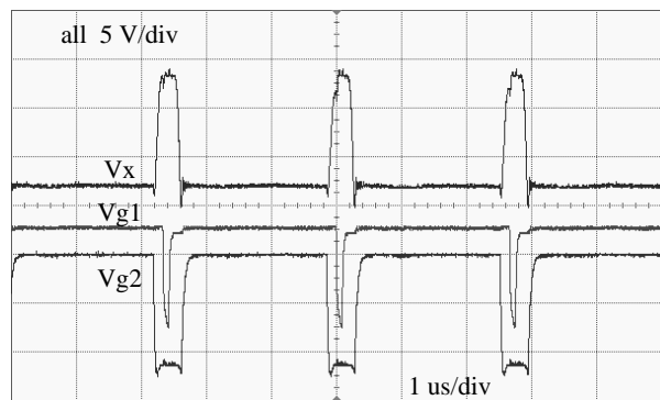
(b) Soft-switching (zero-voltage-switching) behavior ( I_o = 10 A).
