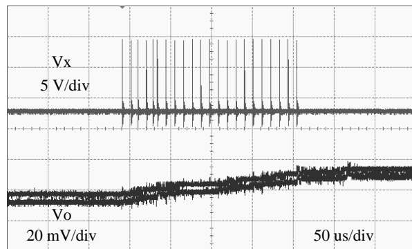
(f) Zoom of single burst in (e); pulse frequency about 94 kHz.
