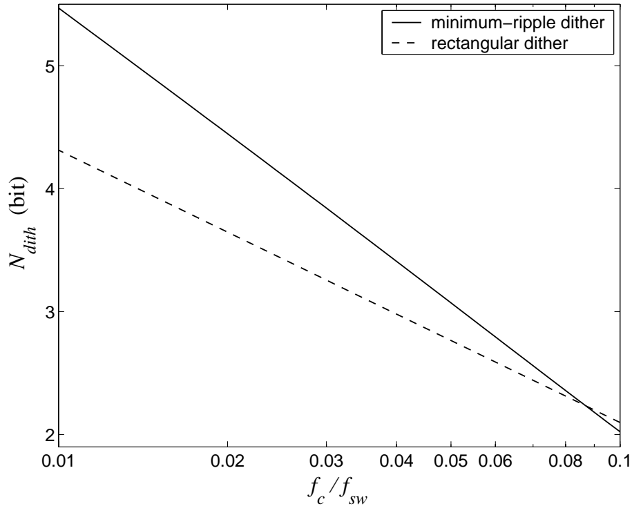
Figure 3.9: Dither bit limit vs. power train cutoff frequency, for f_z = 0.5f_{sw} and \Delta N = 1 .
