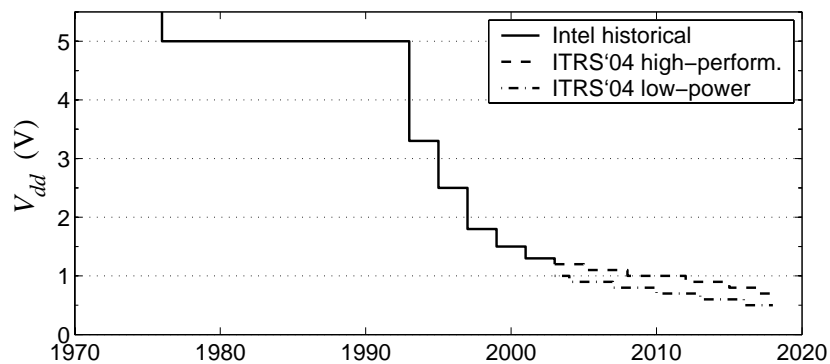
(a) Microprocessor supply voltage. (Sources: [105, 113, 29, 30])
