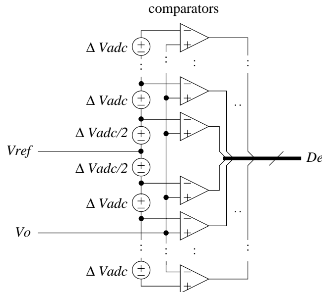
Figure 3.2: Block diagram of a flash window ADC. It implements both an ADC and an error amplifier.
