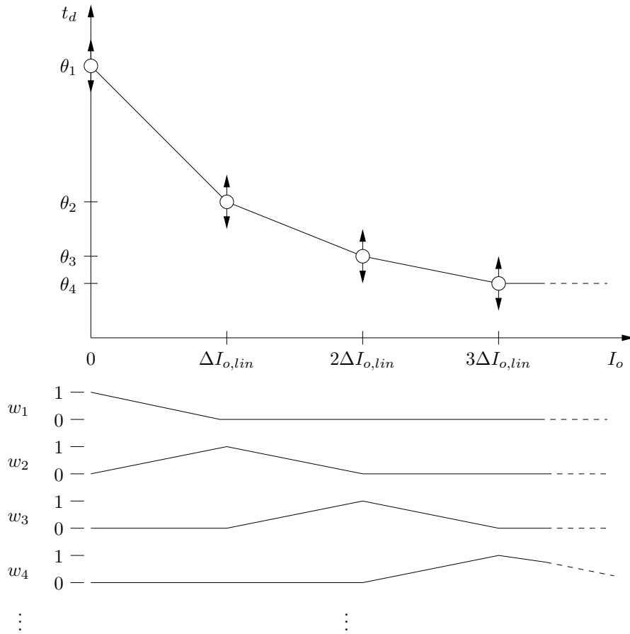
Figure 4.4: Piecewise linear function modeling dead-time t_d(I_o) (top), and associated vertex weights (bottom).
