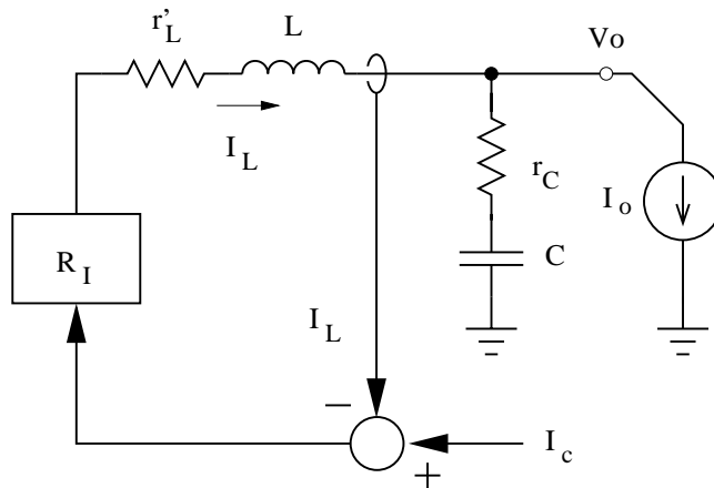
Figure 2.4: Model of current modulator with current (inner) loop closed.
