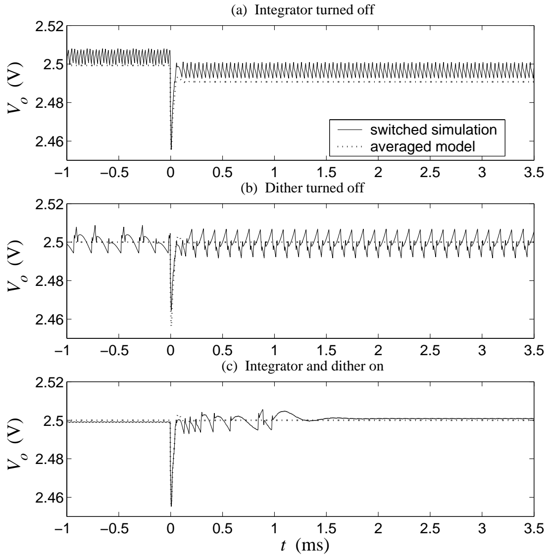
Figure 3.11: Simulated steady-state behavior and transient response of the prototype buck converter with and without integral feedback and dither. Load current steps from 0.5 A to 12 A at t = 0 .
