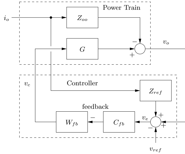
Figure 2.3: Load-line feedback block diagram with voltage-mode control.
