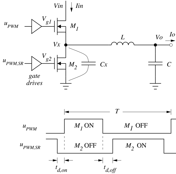
Figure 4.1: Buck converter with synchronous rectifier ( M_2 ), and the corresponding MOSFET control signals.
