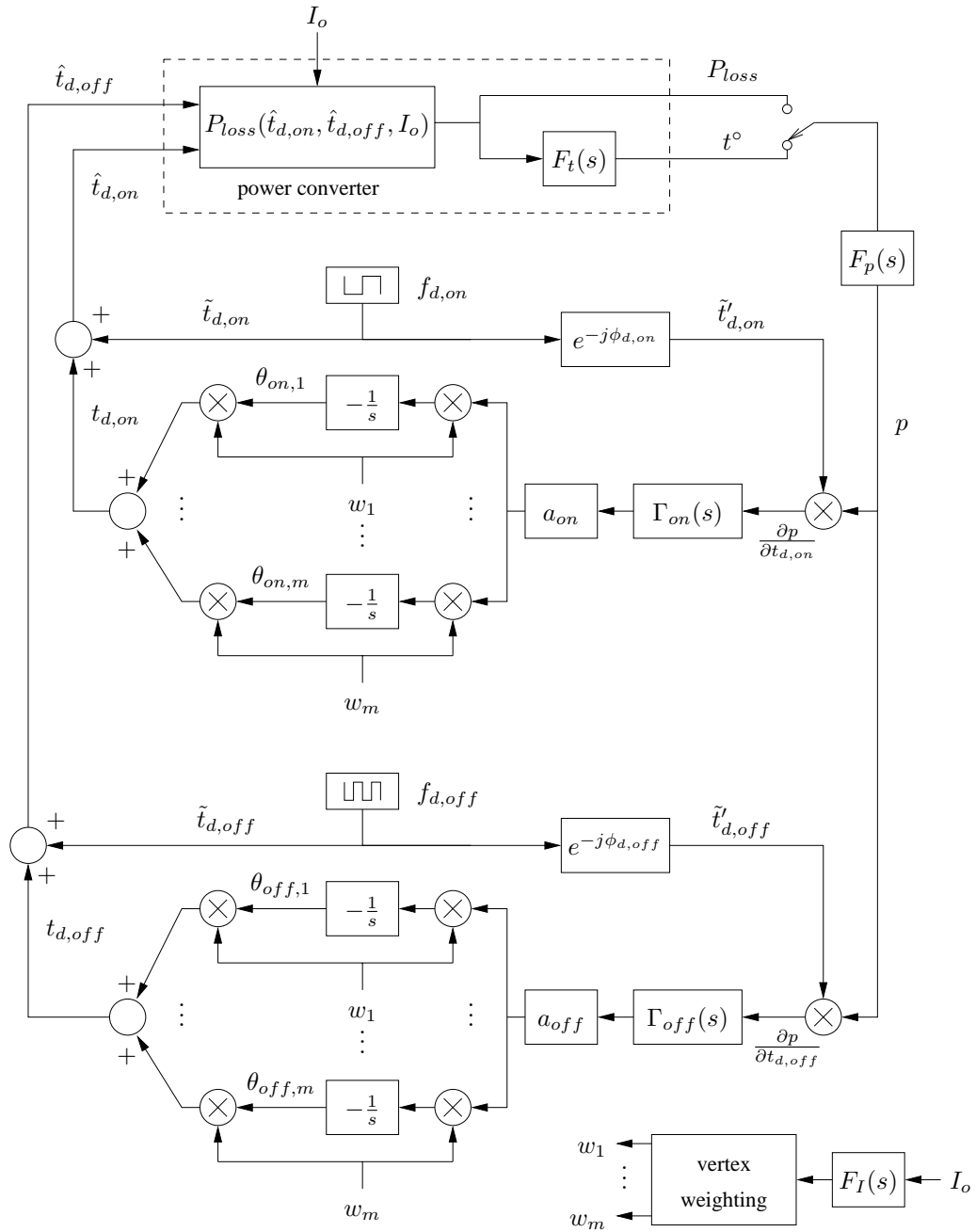
Figure 4.5: Block diagram of synchronous rectifier adaptive control using multi-parameter extremum seeking.
