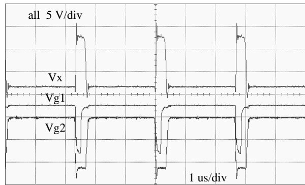
(a) CCM operation ( I_o = 35 A).
