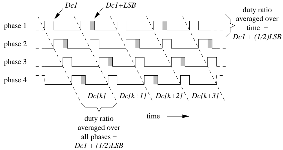
Figure 3.10: Four-phase switching waveform dither patterns implementing a (1/2)LSB effective DPWM level.
