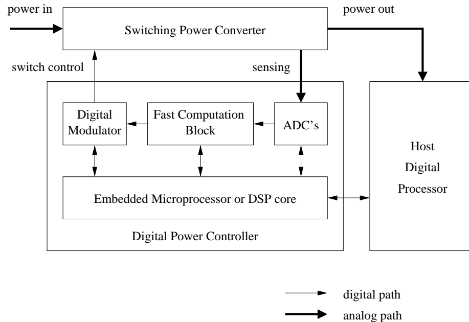
Figure 1.3: Block diagram of a digitally-controlled voltage regulator delivering power to a digital processor.
