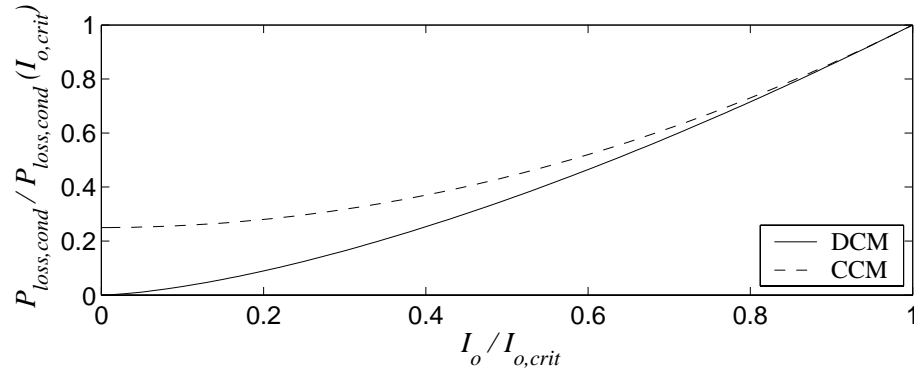
Figure 4.3: Normalized conduction power loss in discontinuous conduction mode (DCM) and continuous conduction mode (CCM).
