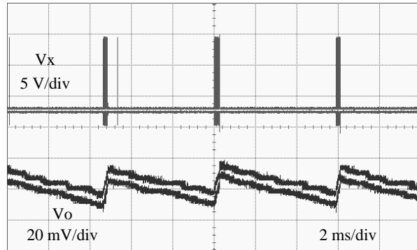
(e) Pulse skipping ( I_o = 0.01 A); bursts repeat at about 170 Hz.
