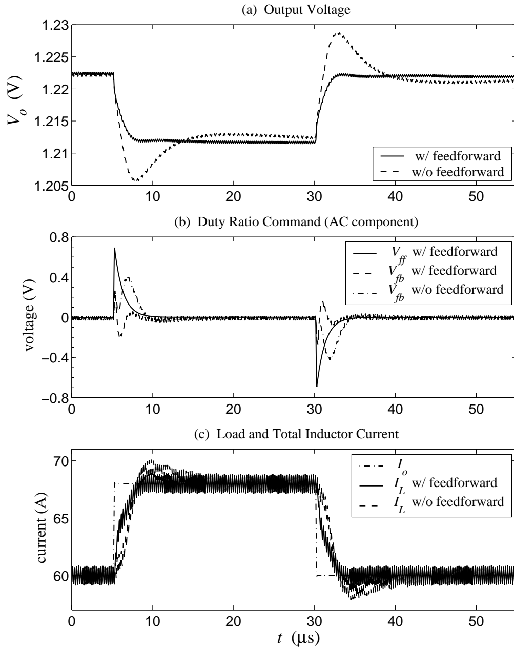
Figure 2.10: Simulated 8 A load transient, from 60 A to 68 A to 60 A, with and without load-current feedforward.
