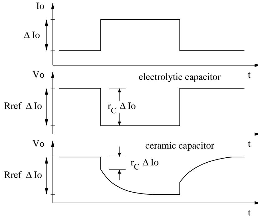
Figure 2.2: Typical current step transient response with load-line regulation, with electrolytic and ceramic capacitors, assuming no duty ratio saturation occurs.
