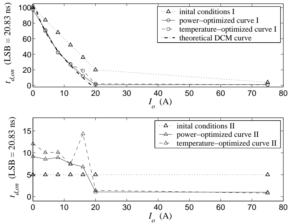
Figure 4.9: Dead-time t_{d,on} versus I_o curves obtained by power loss and temperature minimization experiments for different initial conditions. This is a different representation of the vertical curves in Fig. 4.6.
