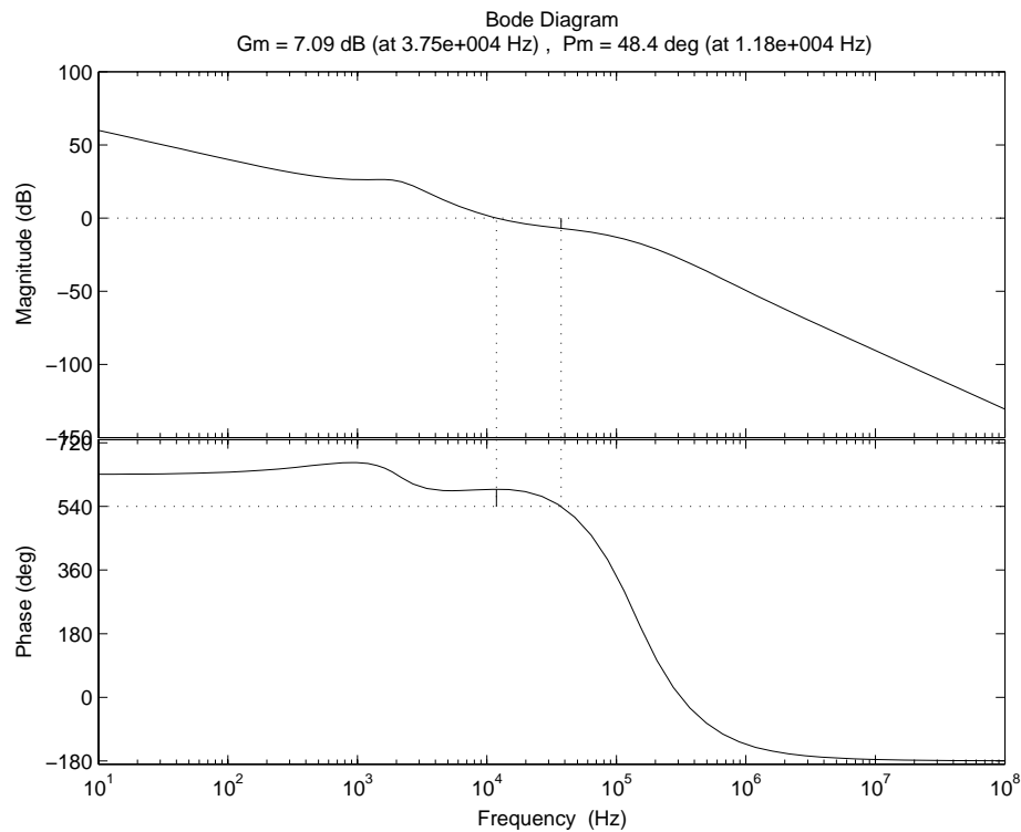
Figure B.1: Converter loop gain calculated with the averaged continuous time model.
