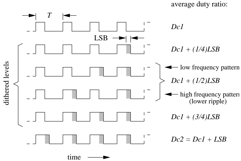
Figure 3.6: Switching waveform dither patterns realizing (1/4)LSB , (1/2)LSB , and (3/4)LSB DPWM effective levels (2-bit dither).
