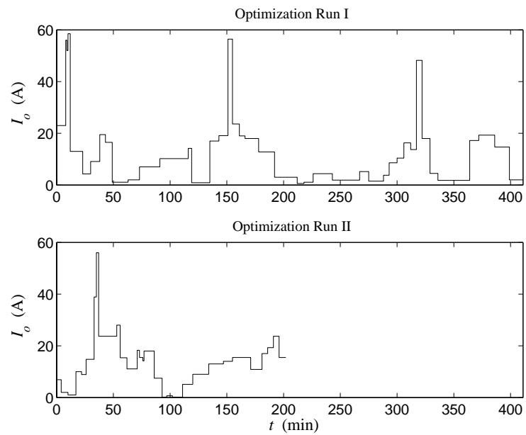
(a) power-loss minimization
