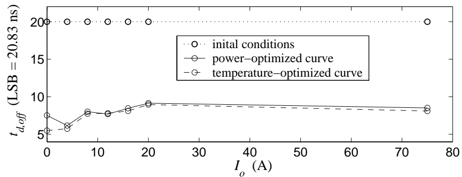
Figure 4.10: Dead-time t_{d,off} versus I_o curves obtained by power loss and temperature minimization experiments. This is a different representation of the vertical curves in Fig. 4.7.
