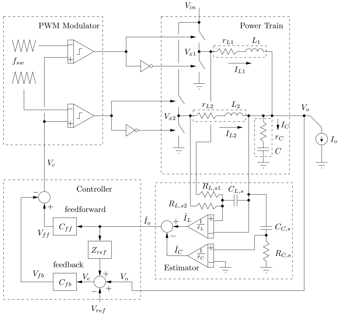
Figure 2.9: Implementation diagram of a two-phase buck converter with load-line regulation and estimated load-current feedforward.
