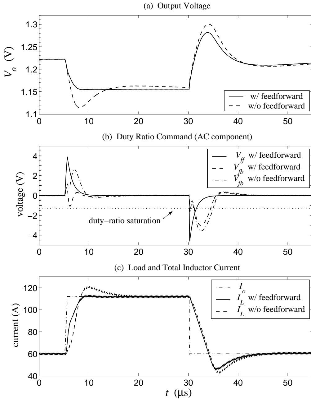
Figure 2.11: Simulated 52 A load transient, from 60 A to 112 A to 60 A, with and without load-current feedforward.
