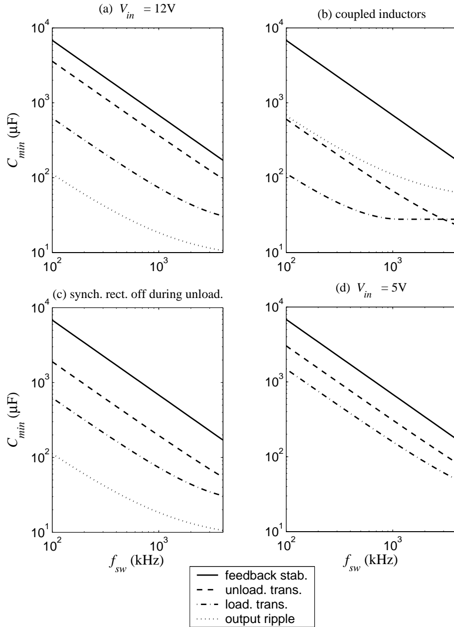
Figure 2.8: Minimum output capacitance constraints associated with unloading and loading transient response, feedback stability, and output ripple. Assumed VR parameters from Table 2.1, and \tau_C = 24 ns, \Delta I_{L\phi,p-p} = 8 A, \Delta V_{o,r,p-p} = 16 mV, V_D = 1 V, t_d = 100 ns, and \alpha = 1/6 .
