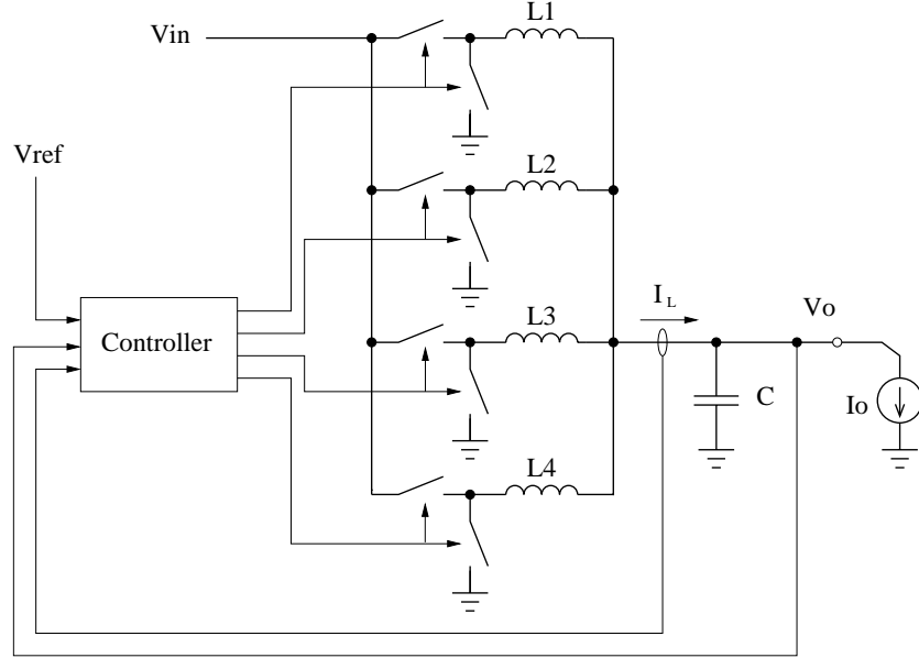
Figure 2.1: Four-phase buck converter. The phases are interleaved at 90^\circ with respect to each other in order to reduce the input-current and output-voltage ripple.
